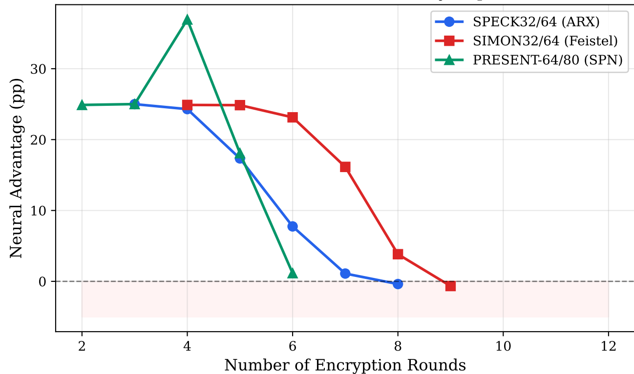
Neural – Classical Accuracy Gap
