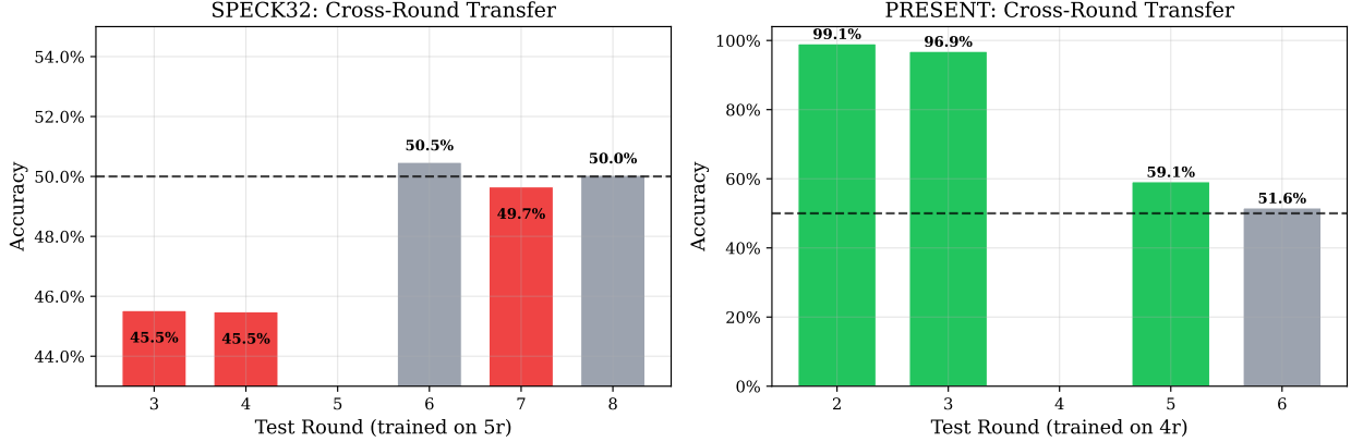
Figure 5: Transfer polarity as a Markov composability test. SPN (PRESENT-64/80) features compose hierarchically: positive transfer confirms Markov-like behavior. ARX (SPECK32/64) and Feistel (SIMON32/64) features anti-compose: accuracy below 50% violates the Markov assumption. Error bars: \pm 1 std over 5 seeds.
