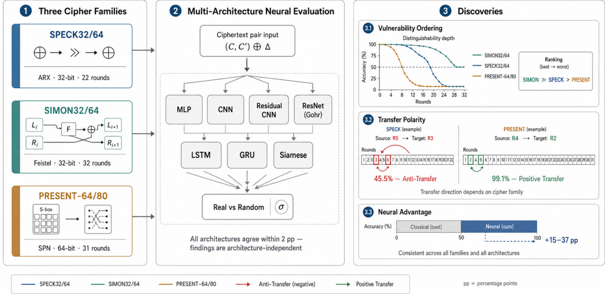
Figure 1: Overview. We train identical neural distinguishers on three cipher families (left) using seven architectures (center) and answer two research questions (right). RQ1: Signal resides in XOR-difference bits and is architecture-independent—all models agree within 2 pp, establishing a vulnerability ordering SIMON32/64 \gg SPECK32/64 > PRESENT-64/80. RQ2: Signal composition is family-dependent—SPN features compose hierarchically (positive transfer >99%), while ARX/Feistel features anti-compose (<50%), violating the Markov assumption that underlies classical differential analysis.
