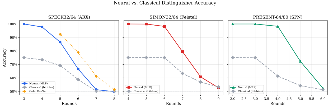
Figure 3: Neural (MLP) vs. classical (best-bit-bias) accuracy across rounds. The neural advantage is largest at intermediate rounds, where multi-bit correlations are strongest, and collapses at the boundary.
