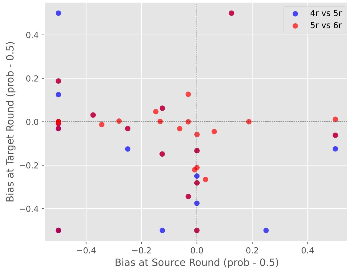
Bit-Bias Oscillation in Simon32/64
