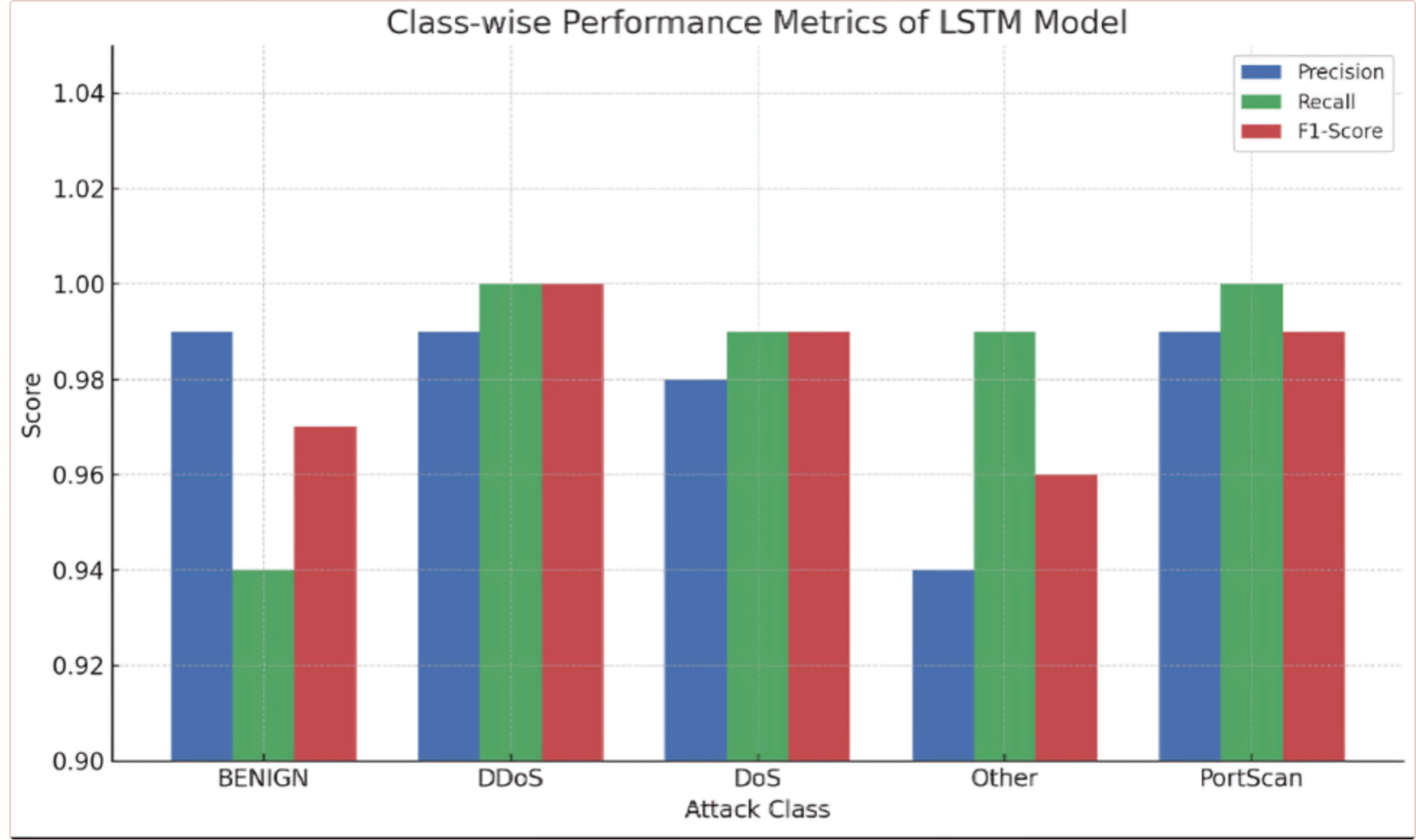
Fig. 5 – Class-wise Performance
