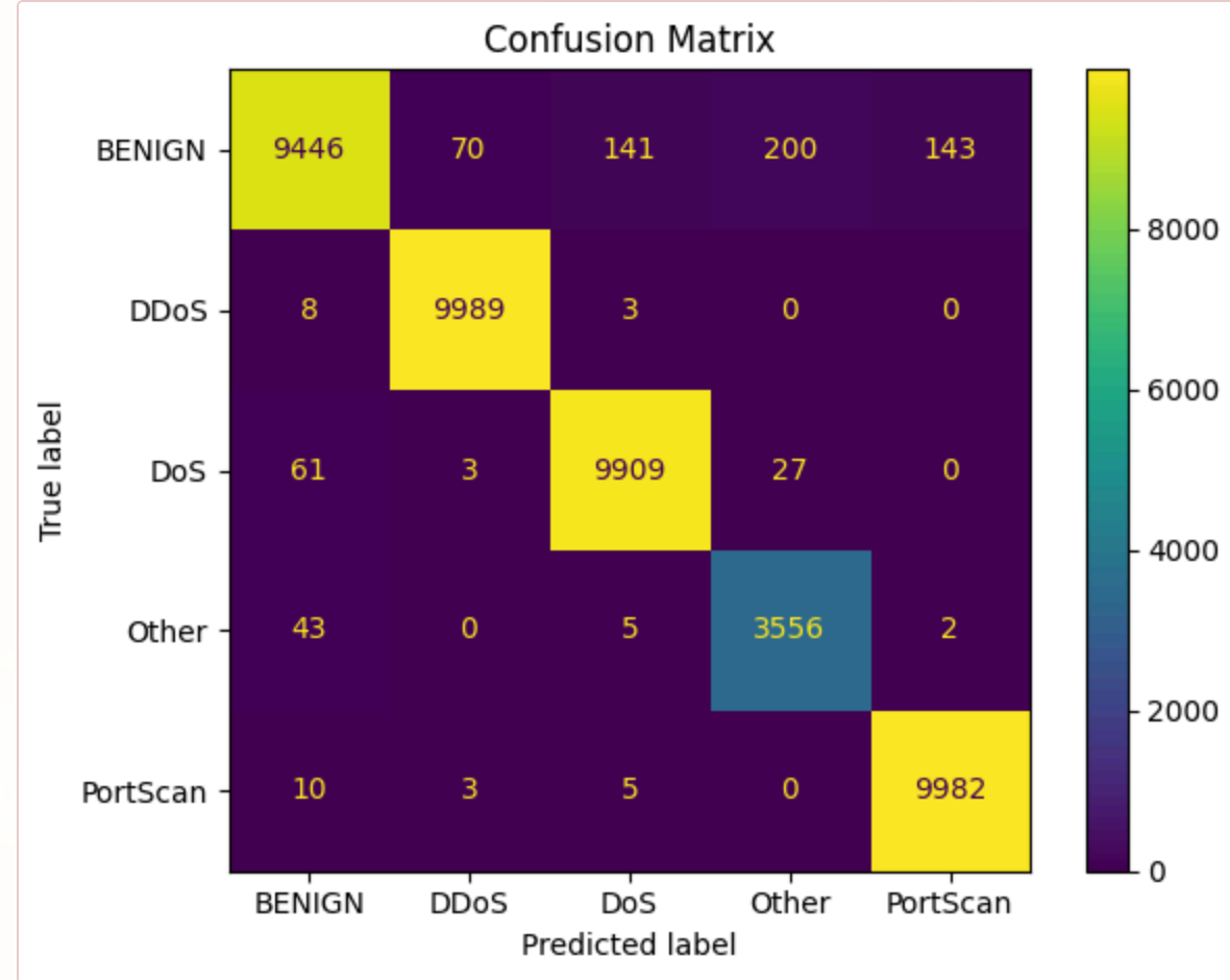
Fig. 4 – Confusion Matrix
