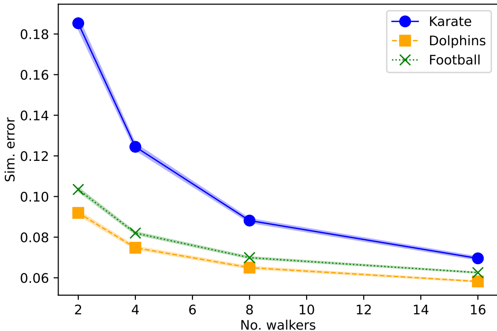
Diffusion simulation error vs. no. walkers
