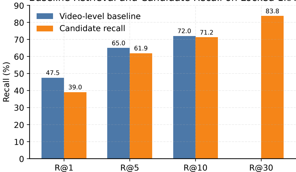
Baseline Retrieval and Candidate Recall on Locked 1kA
