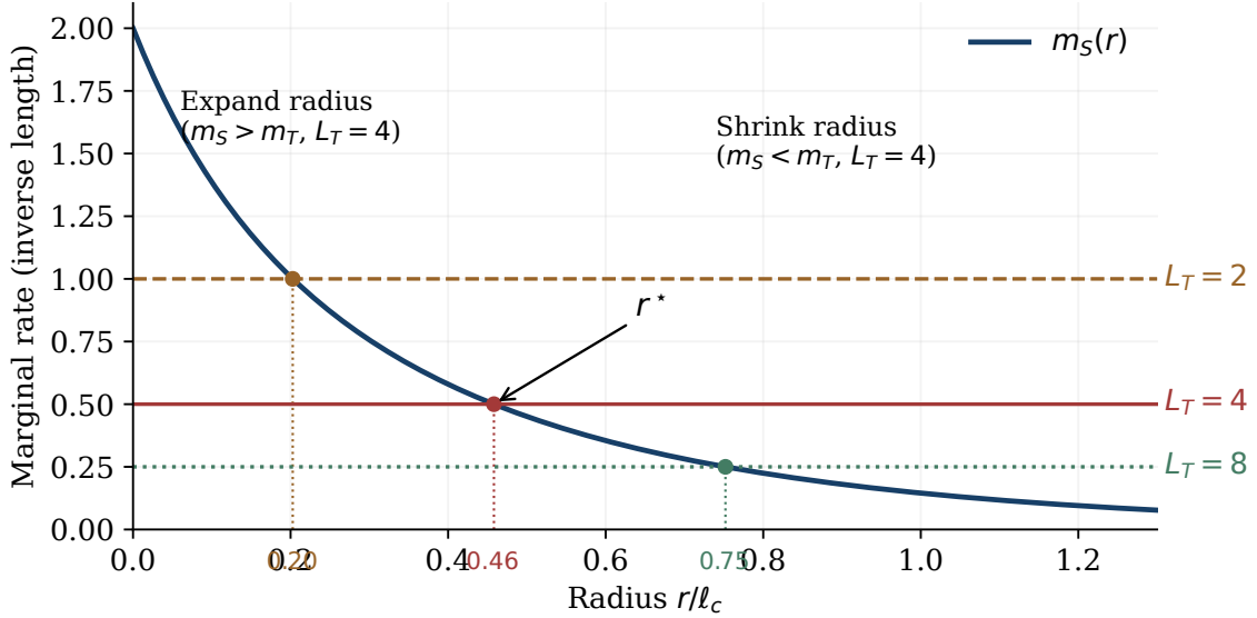
Figure 2: Marginal balance in the canonical model with \ell_c = 1 and \ell_s = 0.5 . Increasing L_T = vT lowers m_T = 2/L_T and moves the crossing with m_S outward. For the middle curve ( L_T = 4 ), regret falls to the left of the crossing and rises to its right. This is an illustration of the analytical rates, not an additional numerical experiment.
