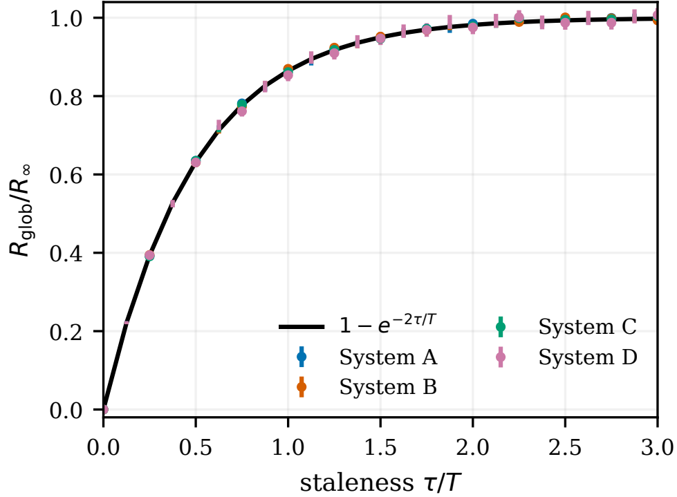
Figure 3: Temporal scaling collapse from exact stationary OU pairs. Markers are Monte Carlo estimates for four systems with different dimensions, spatial covariances, objective matrices, and decision operators; bars are 95% confidence intervals. The solid curve is the exact law 1 - e^{-2\tau/T} . Normalization by R_\infty removes system-specific scale.
