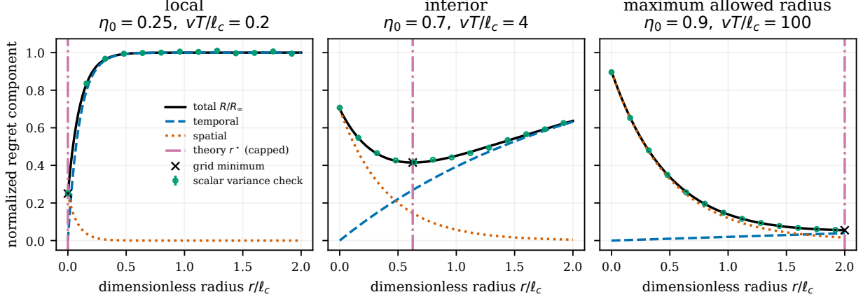
Figure 5: Emergence of local, interior, and maximum allowed radius optima under \eta_S(r) = \eta_0 e^{-2r/\ell_c} and \tau(r) = r/v . Curves show total regret and its temporal and residual-spatial terms from Eq. (91); open markers with 95% intervals are independent scalar-innovation estimates. Dash-dotted lines and crosses mark the analytical constrained and grid minimizers. At the maximum allowed radius, positive omission remains: \eta_S(D) > 0 .
