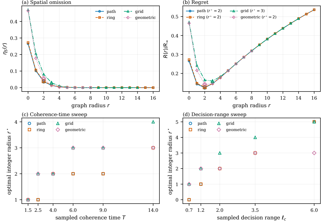
Figure 8: Finite noncanonical graphs. Top: \eta_S(r) computed from exact Gaussian conditional covariances and the resulting regret under one common normalized setting; lines join integer-radius evaluations. Bottom: exact integer optima at the sampled coherence times and decision ranges; no transition locations between those settings are inferred. Distinct marker shapes identify coincident graph results. The canonical line closed form is not used.
