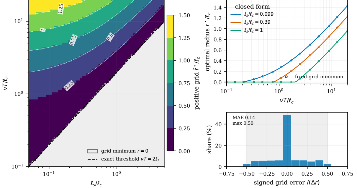
Figure 6: Dimensionless optimal-radius law from direct scalar minimization. Left: the numerical map, with the numerical zero-radius region shown in gray and the dashed curve marking the theoretical transition vT = 2\ell_s . Upper right: selected \ell_s/\ell_c slices comparing grid minimizers with the closed form in Eq. (109). Lower right: the histogram of (\hat{r}^* - r^*)/\Delta r over all 4,896 points; its zero spike includes local-regime points and the remaining grid errors are of order a half-step.
