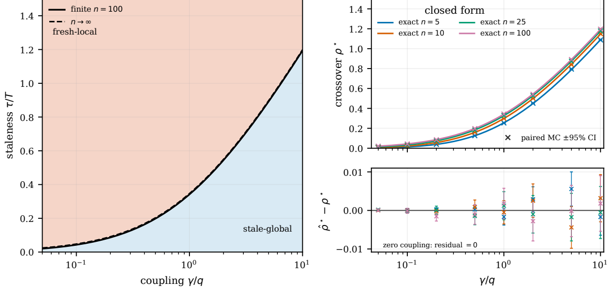
Figure 4: Fresh-local versus stale-global crossover. Left: the phase map uses the exact finite- n = 100 boundary (solid) and the large- n limit (dashed), Eqs. (62) and (64). Upper right: exact theory curves and inferred Monte Carlo boundaries (crosses) for four system sizes, with paired delta-method 95% intervals. Lower right: empirical minus theoretical boundary, on a scale that reveals the sampling differences and their uncertainty. The zero-coupling setting is evaluated at \rho^* = 0 but omitted from the logarithmic positive-coupling axes.
