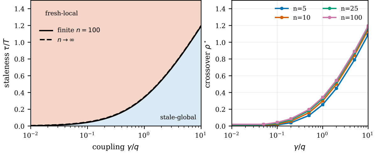
Figure 2: Fresh-local versus stale-global crossover. Left: winning architecture for n = 100 ; the solid finite- n boundary and dashed large- n boundary are Eqs. (67) and (69). Right: covariance boundaries (lines) and Monte Carlo estimates (crosses) for four system sizes. Stronger coupling makes older global information worth tolerating.
