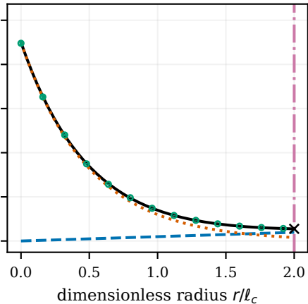
maximum allowed radius \eta_0 = 0.9, \nu T/\ell_c = 100
