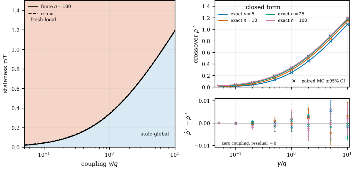
Figure 2: Fresh-local versus stale-global crossover. Left: the phase map uses the exact finite- n = 100 boundary (solid) and the large- n limit (dashed), Eqs. (49) and (51). Upper right: exact theory curves and inferred Monte Carlo boundaries (crosses) for four system sizes, with paired delta-method 95% intervals. Lower right: empirical minus theoretical boundary, on a scale that reveals the sampling differences and their uncertainty. The zero-coupling setting is evaluated at \rho^* = 0 but omitted from the logarithmic positive-coupling axes.
