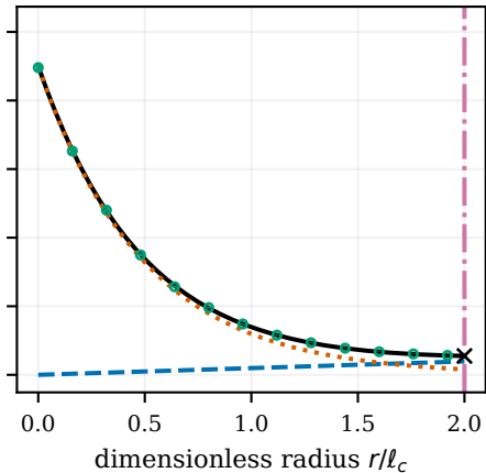
boundary (capped maximum) \eta_0 = 0.9, \nu T/\ell_c = 100
