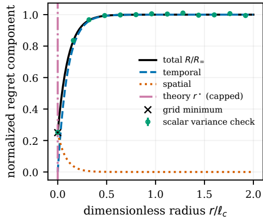
local \eta_0 = 0.25, \nu T/\ell_c = 0.2
