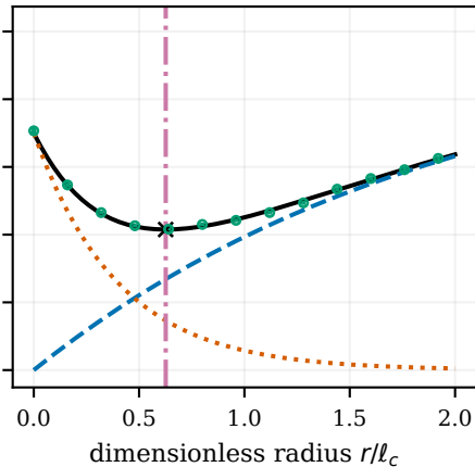
interior \eta_0 = 0.7, \nu T/\ell_c = 4
