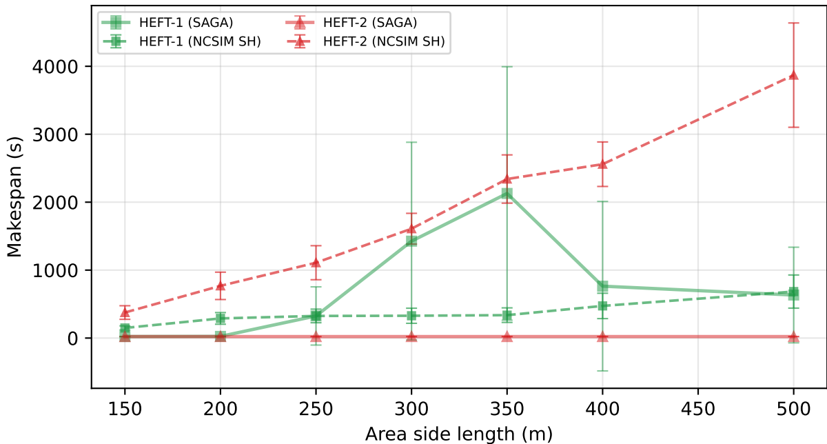
Random — Large DAG — SAGA vs NCSIM (SH)
