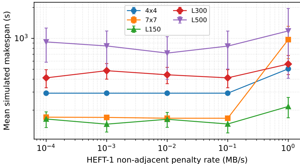
HEFT-1 penalty sensitivity (large DAG, SH routing)
