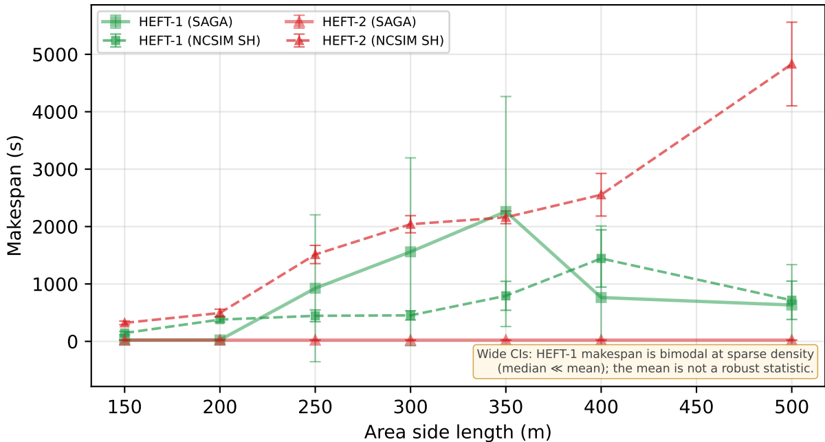
Random — Large DAG — SAGA vs NCSIM (SH), 95% CI
