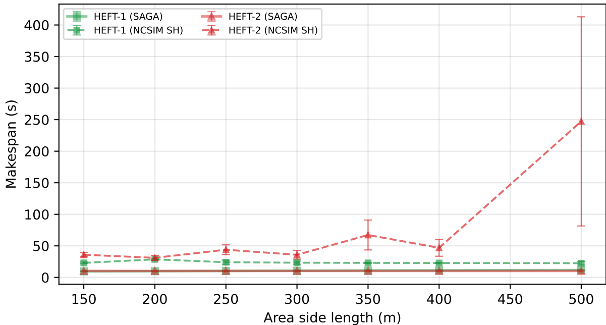
Random — Small DAG — SAGA vs NCSIM (SH), 95% CI
