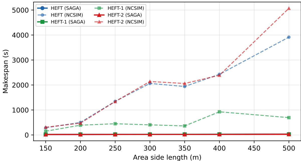
Random — Large DAG — SAGA vs NCSIM
