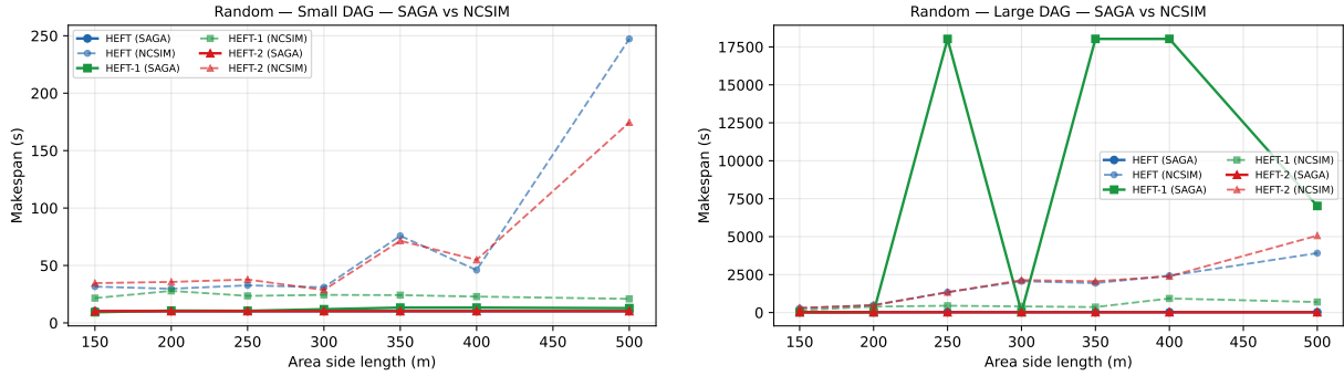
Figure 4: SAGA predicted (solid) vs NCSIM best-routing simulated (dashed) makespan vs density. SAGA’s HEFT-2 estimate stays low regardless of density; NCSIM shows HEFT-2 degrading rapidly at low density (longer paths accumulate more interference). HEFT-1’s SAGA estimate is more pessimistic but closer to the actual NCSIM result.
