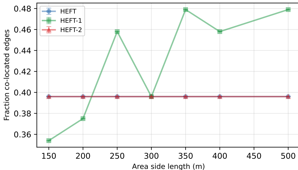
Large DAG — Fraction co-located edges
