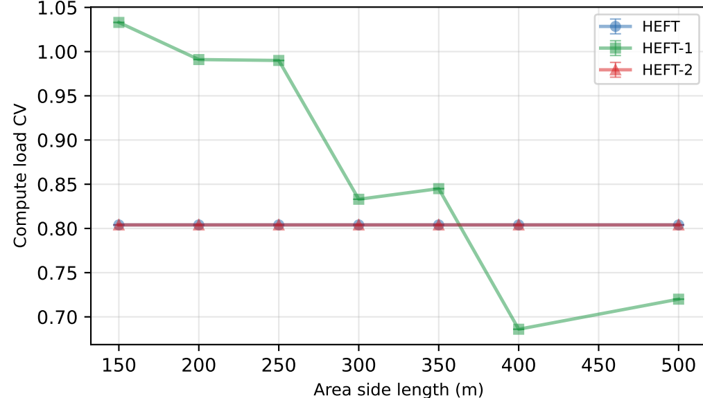
Large DAG — Compute load CV
