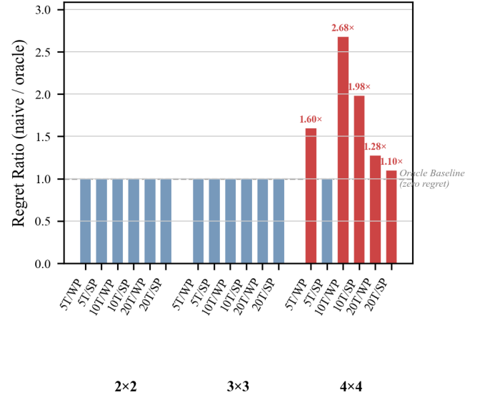
Fig. 8: Scheduling regret ratios. Each bar shows the ratio of the interference-free-optimal makespan (scheduler chosen under the interference-free model, run under the interference-aware model) to the oracle makespan (best scheduler under interference). A ratio of 1.0 indicates zero regret; red bars mark rank inversions where the interference-free choice is suboptimal.
