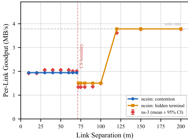
(b) Separation Sweep
