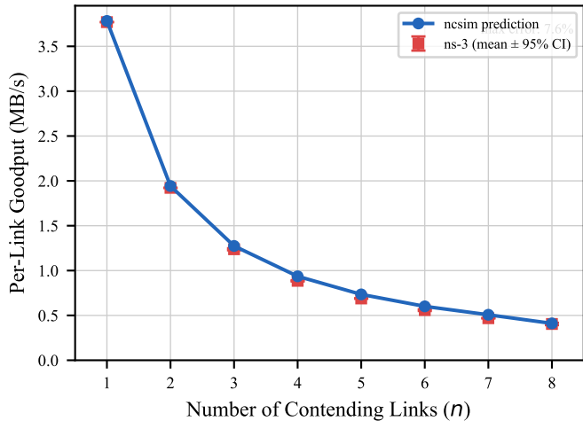
(a) Contention Scaling
