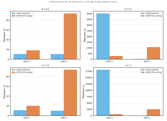
Fig. 1. HEFT analytic prediction (blue) vs. ncsim simulated makespan with SH routing (orange) for the four grid configurations of Table III. Each panel uses its own y -axis scale; the prediction–simulation gap inverts the HEFT1/HEFT2 ranking on both large-DAG cases.
