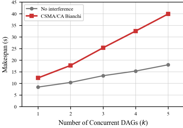
Fig. 10: Multi-DAG makespan scaling on 3 \times 3 grid (5-task DAGs, HEFT, shortest-path). Contention amplifies super-linearly: the gap between the curves widens from 1.47\times ( k=1 ) to 2.21\times ( k=5 ).
