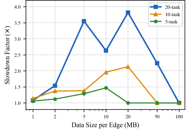
Fig. 9: Interference slowdown vs. data size per edge ( 3 \times 3 grid, HEFT, shortest-path). Slowdown peaks at intermediate CCR values where transfers are long enough to contend but not so large that the scheduler collapses tasks onto one node.
