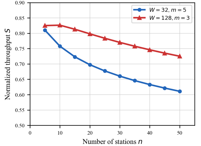
Fig. 5: Reproduction of Bianchi [9] Figure 6: normalized saturation throughput vs. number of stations for two (W, m) configurations. Computed using Bianchi’s exact FHSS parameters (1 Mbps basic access, no RTS/CTS). The W=128 curve’s slight non-monotonicity between n=5 and n=10 is consistent with Bianchi’s published results.
