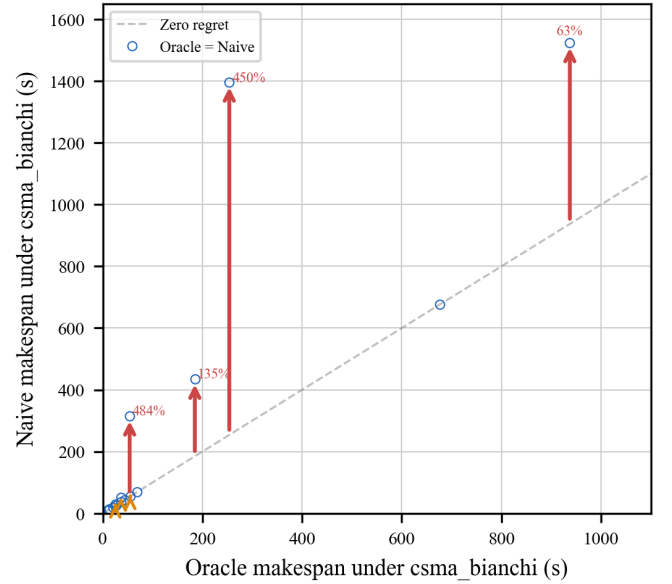
Fig. 7: Makespan regret scatter plot. Each arrow connects the oracle makespan (best scheduler under csma_bianchi) to the naive makespan (scheduler chosen under interference-free model, run under csma_bianchi). Red arrows indicate rank inversions; orange arrows indicate moderate regret. 7 of 18 triples exhibit rank inversions.
