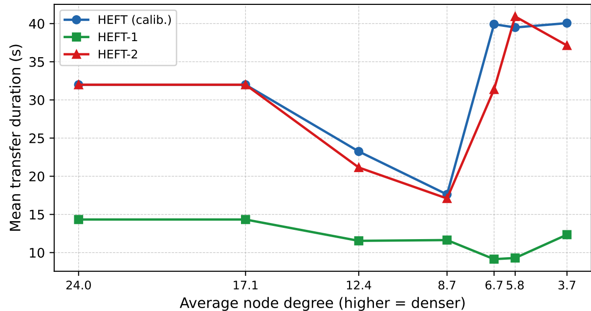
Large DAG — Mean transfer duration vs.\ density
