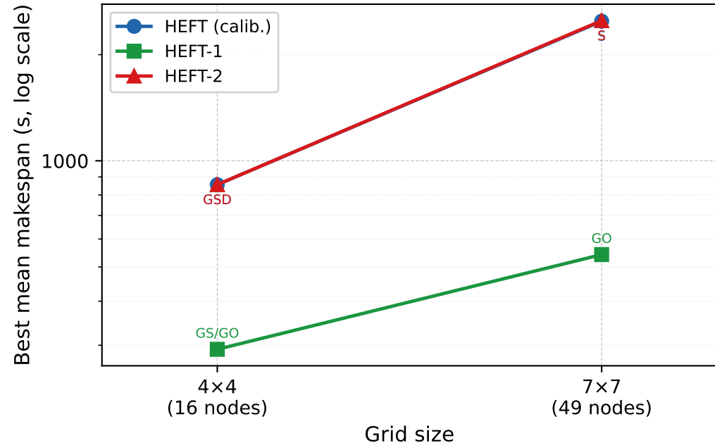
Large DAG (30/60 tasks, pipeline)
