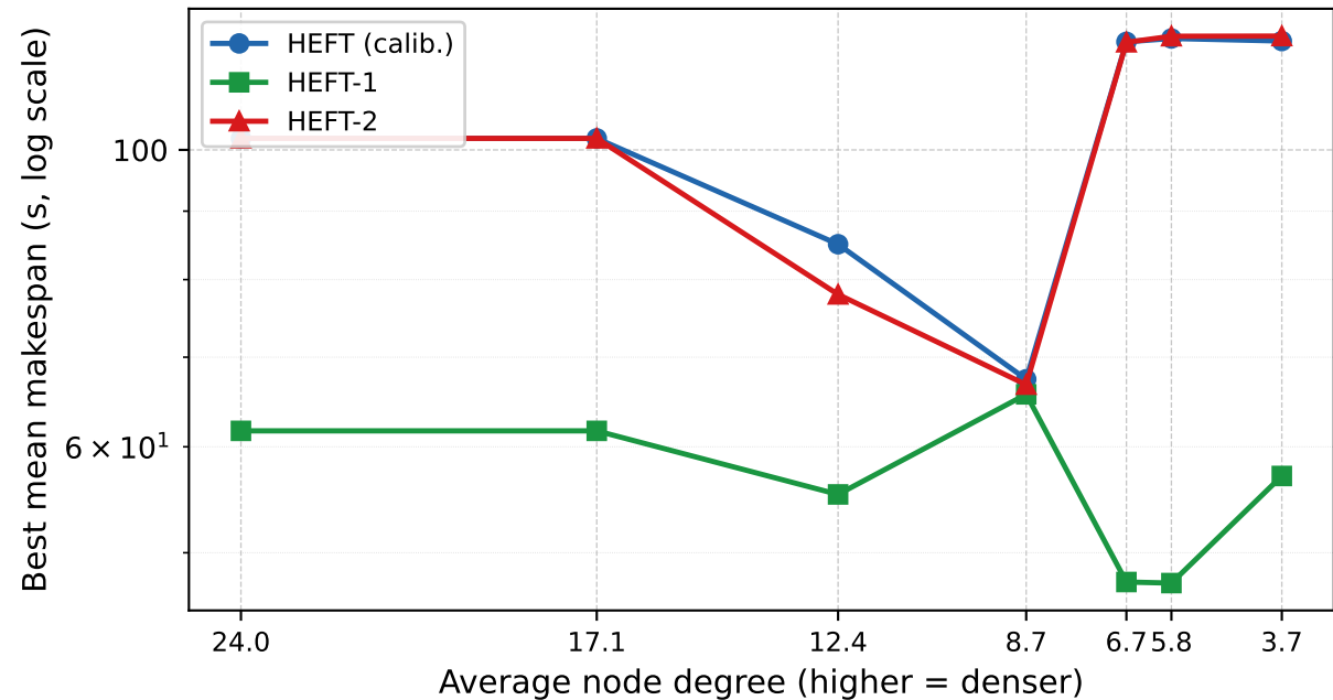
Large DAG (30 tasks, 5-stage pipeline)
