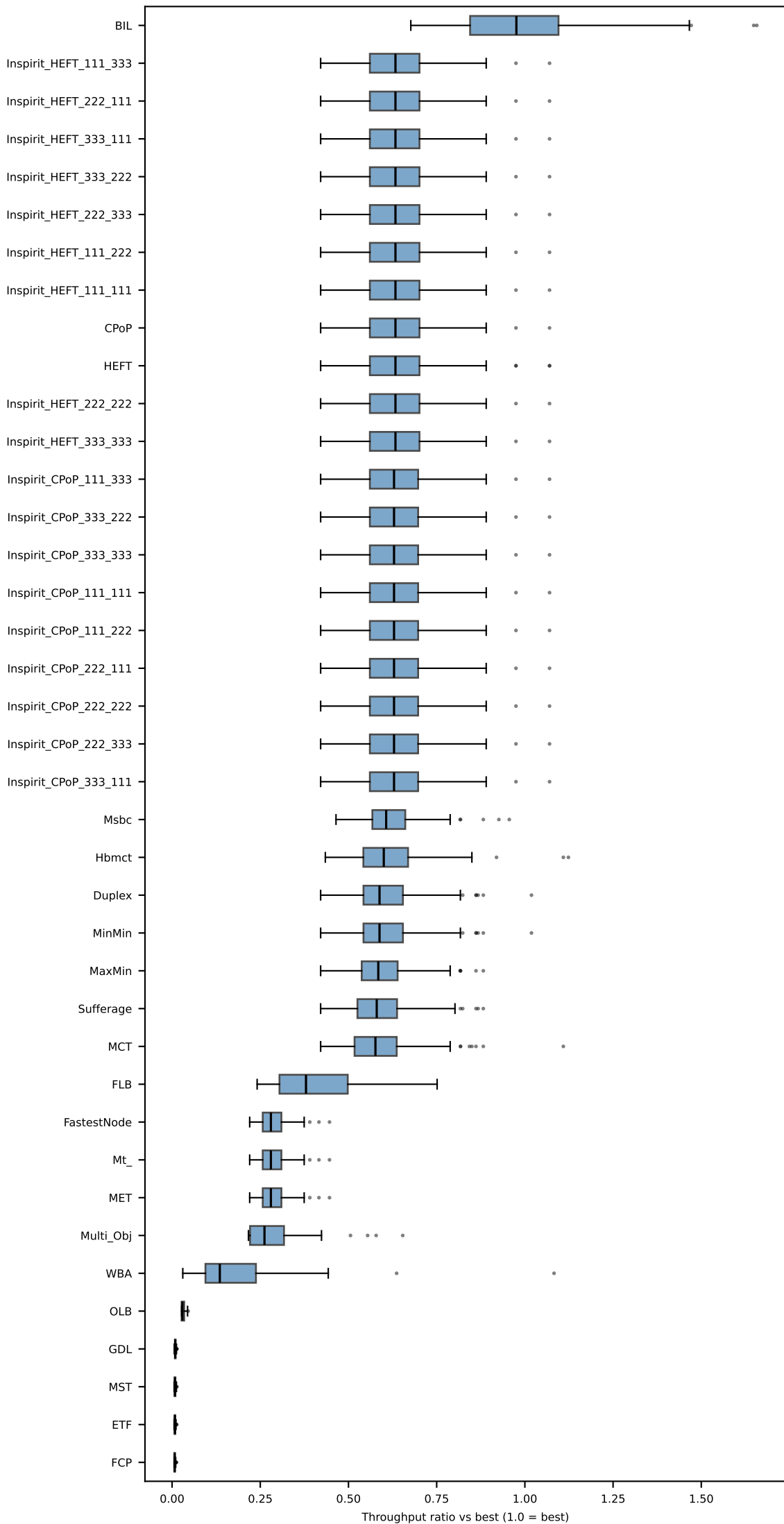
Throughput Benchmarking — train
