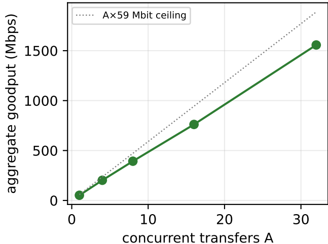
(a) Part C — goodput
