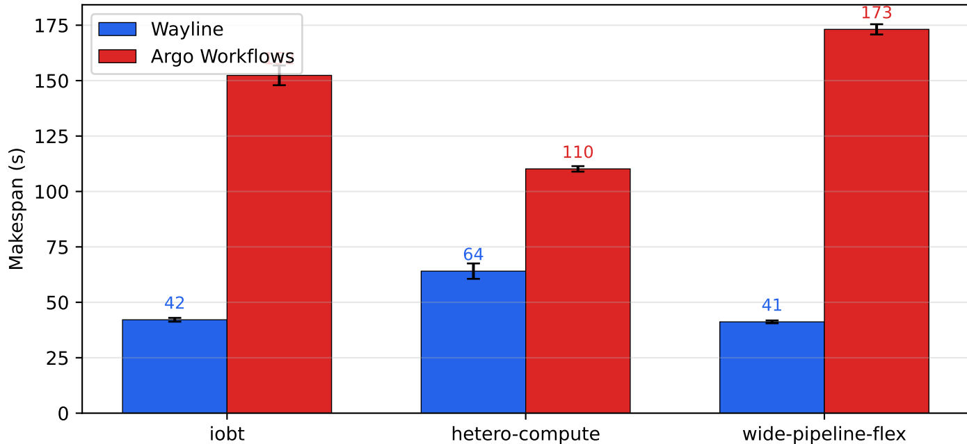
E1 — End-to-end makespan, Wayline vs Argo Workflows (warm window, N=16)
