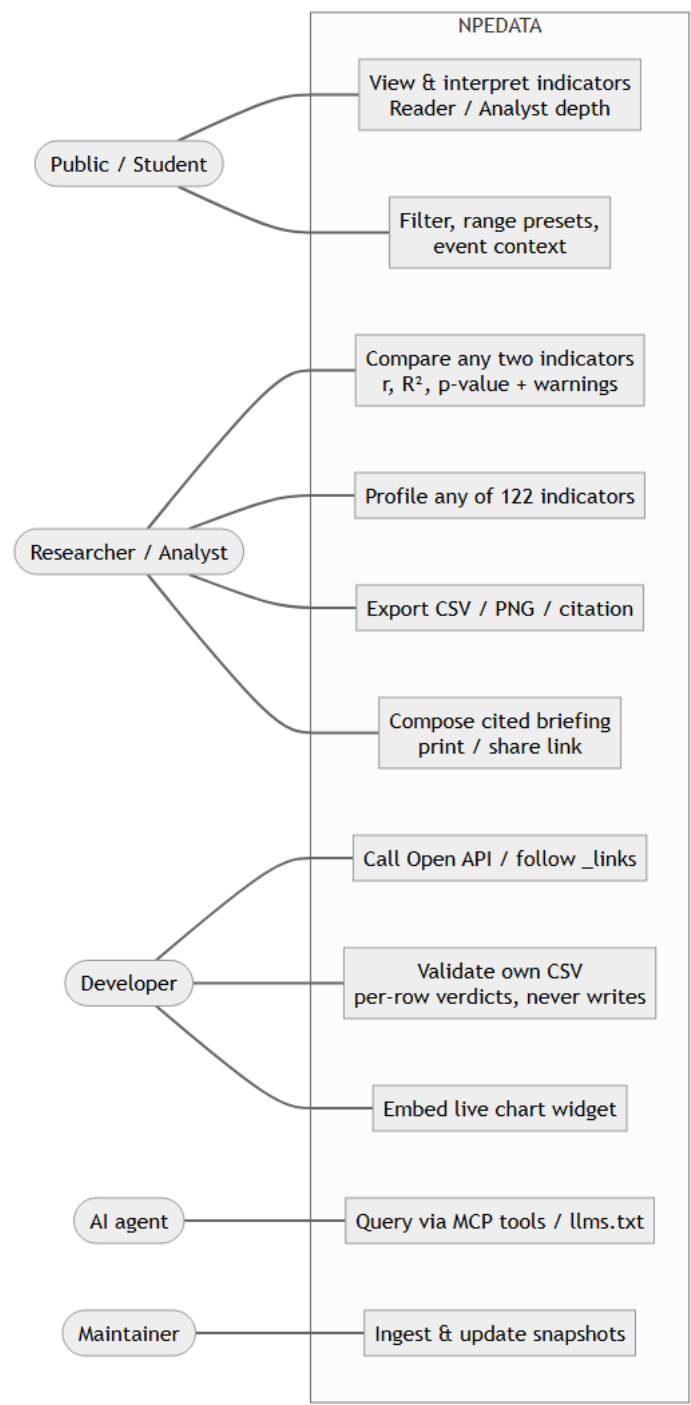
Figure 3.3, Use-case diagram
