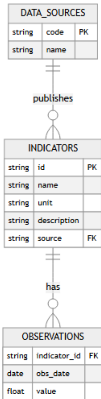
Figure 3.5, Entity-relationship diagram
