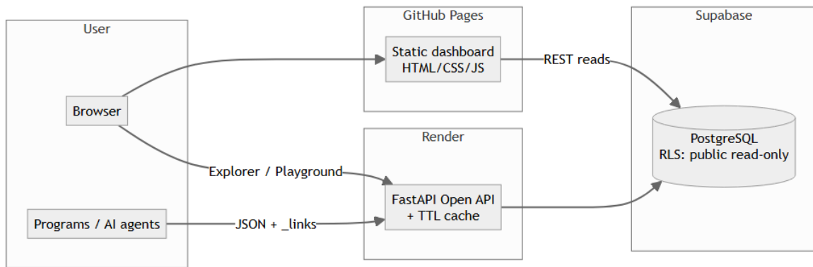
Figure 3.2, Deployment view
