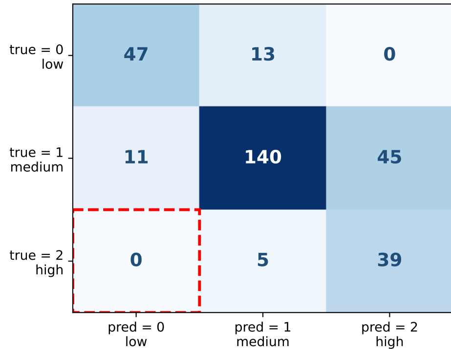
Qwen3-8B issue-only (within-model, primary; \kappa = 0.572 )
