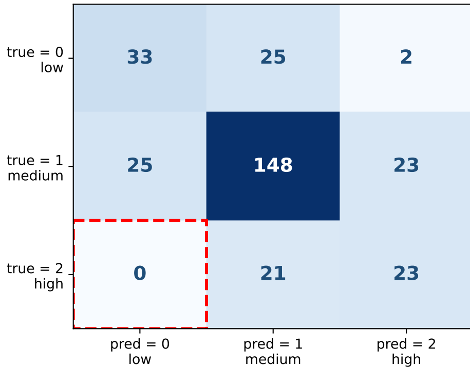
Claude Sonnet 4.5 issue-only (cross-model; \kappa = 0.379 )
