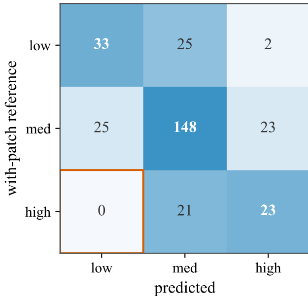
Claude issue-only ( \kappa = 0.379 )
