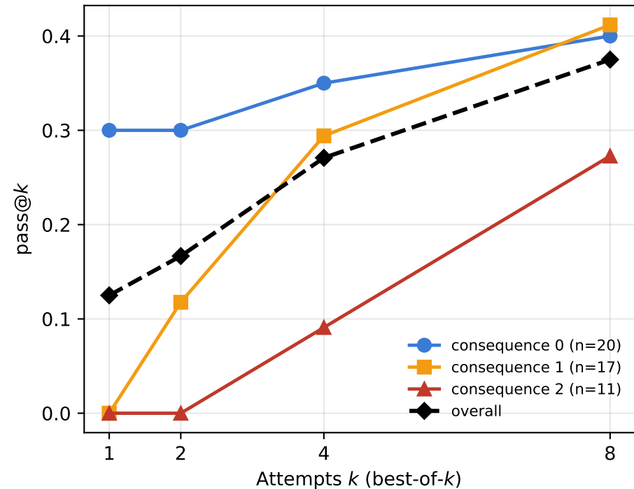
Within-model headroom: pass@k rises with attempts
