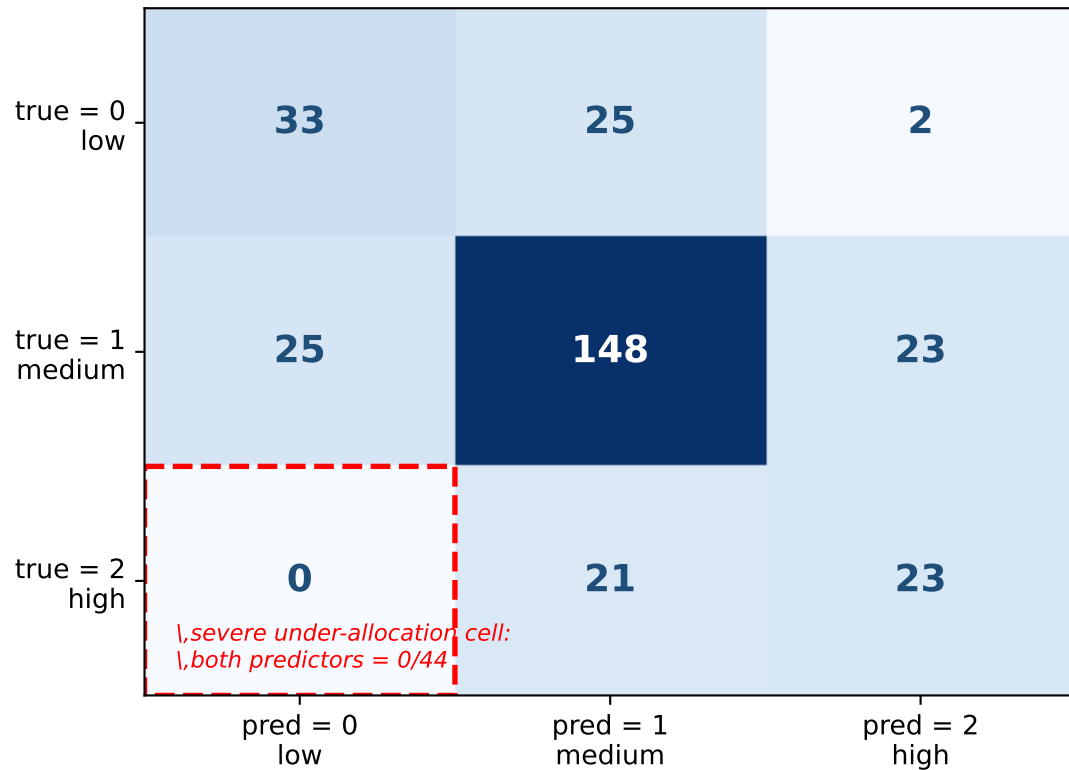
Claude Sonnet 4.5 issue-only (cross-model; \kappa = 0.379 )
