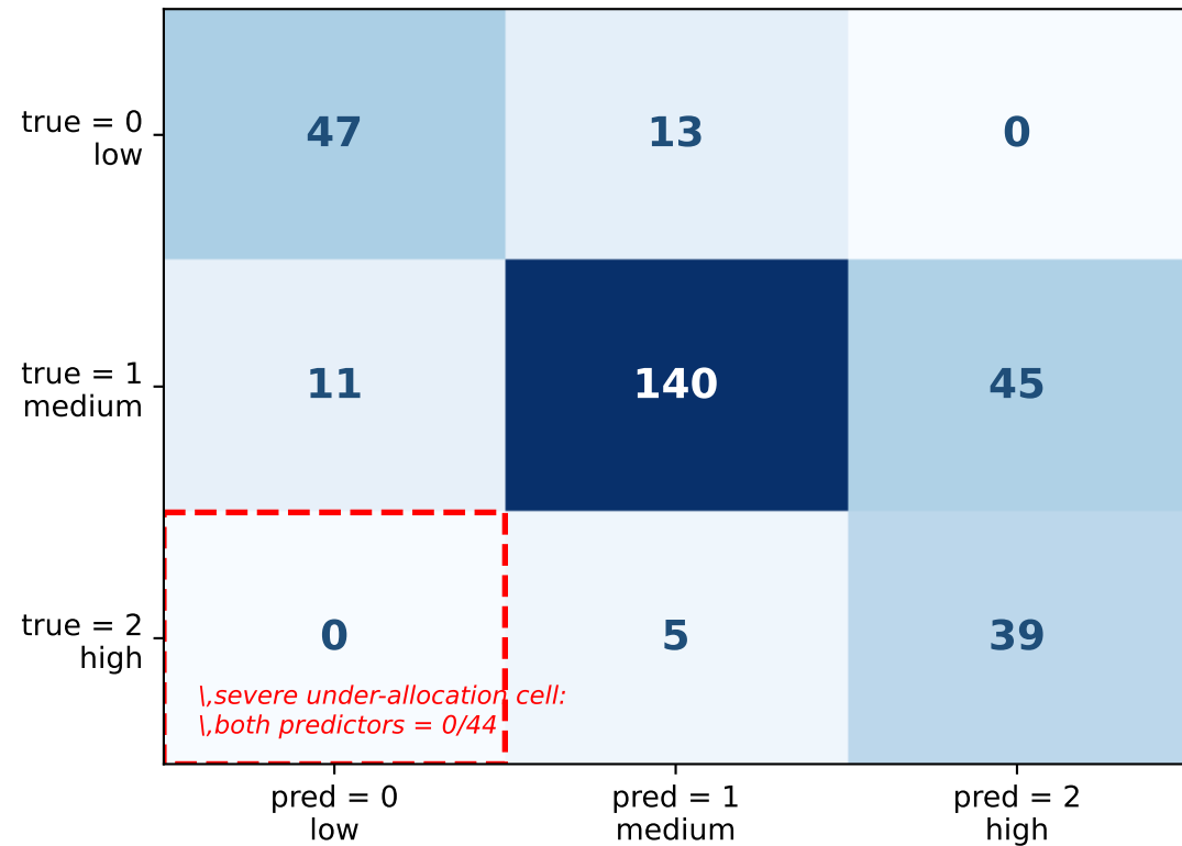
Qwen3-8B issue-only (within-model, primary; \kappa = 0.572 )
