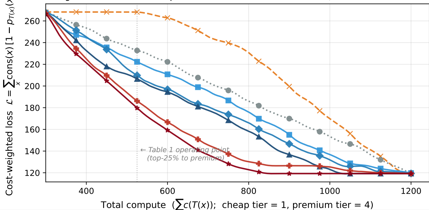
Cost-weighted loss vs total compute on 300 SWE-bench Lite tasks (16-model tier benchmark)
