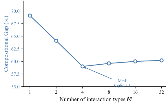
Figure 7: Sensitivity to M . Gap follows a U-shape: M=4 is optimal, with mild increase for M>8 .
