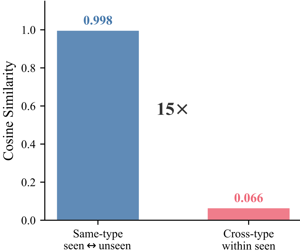
Figure 6: Representation specialization. Left: per-type cosine similarity between seen and unseen activations (all >0.995 ). Red dashed line shows cross-type mean (0.066). Right: the 15\times gap between same-type and cross-type similarity confirms typed modules learn specialized, non-overlapping mechanisms.
