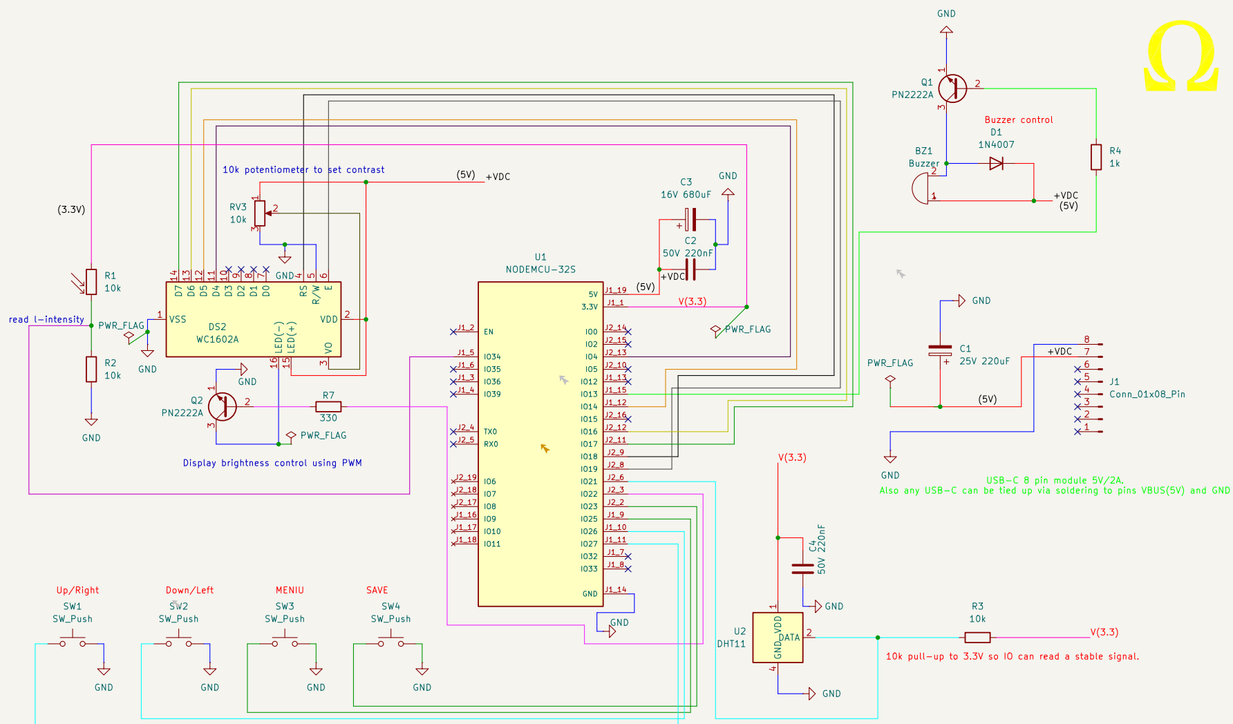
Complete thermostat unit schematic, all analog devices + digital IC.
