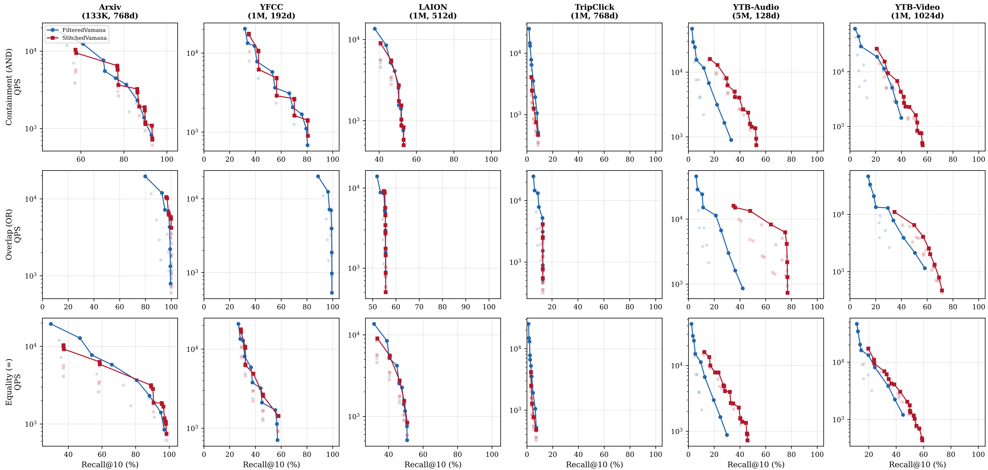
Recall@10 vs QPS: Original Labels (3 Scenarios × 6 Datasets)
