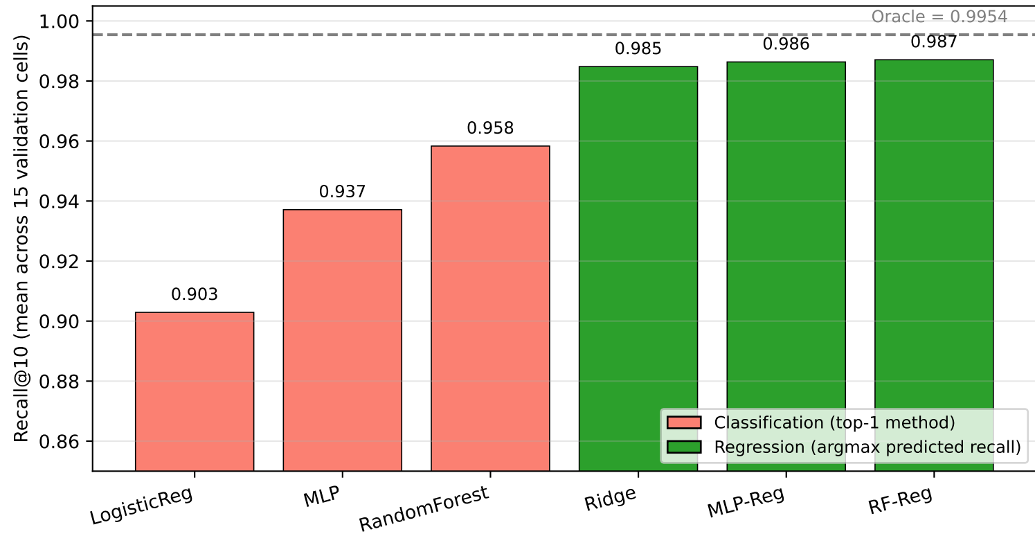
Classification vs Regression Router (plain argmax, validation set)
