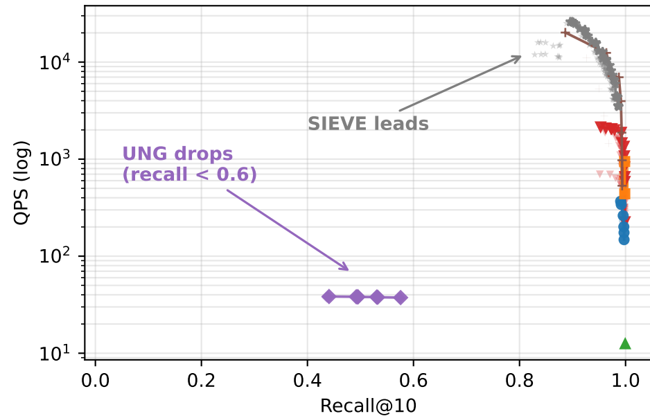
YFCC / OR (Overlap)
