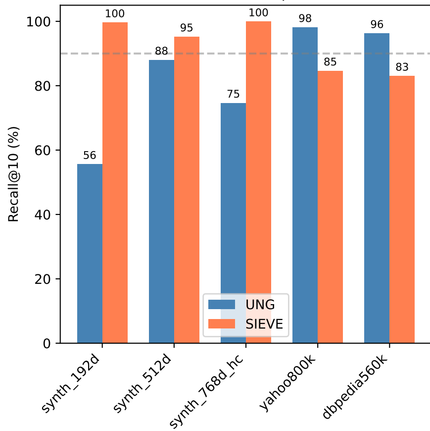
OR (Overlap)
