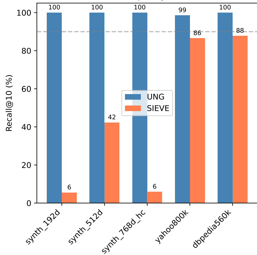
Equality
