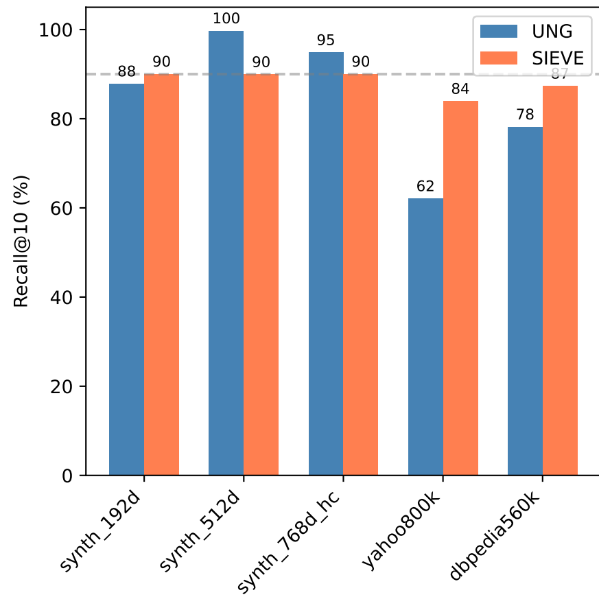
AND (Containment)
