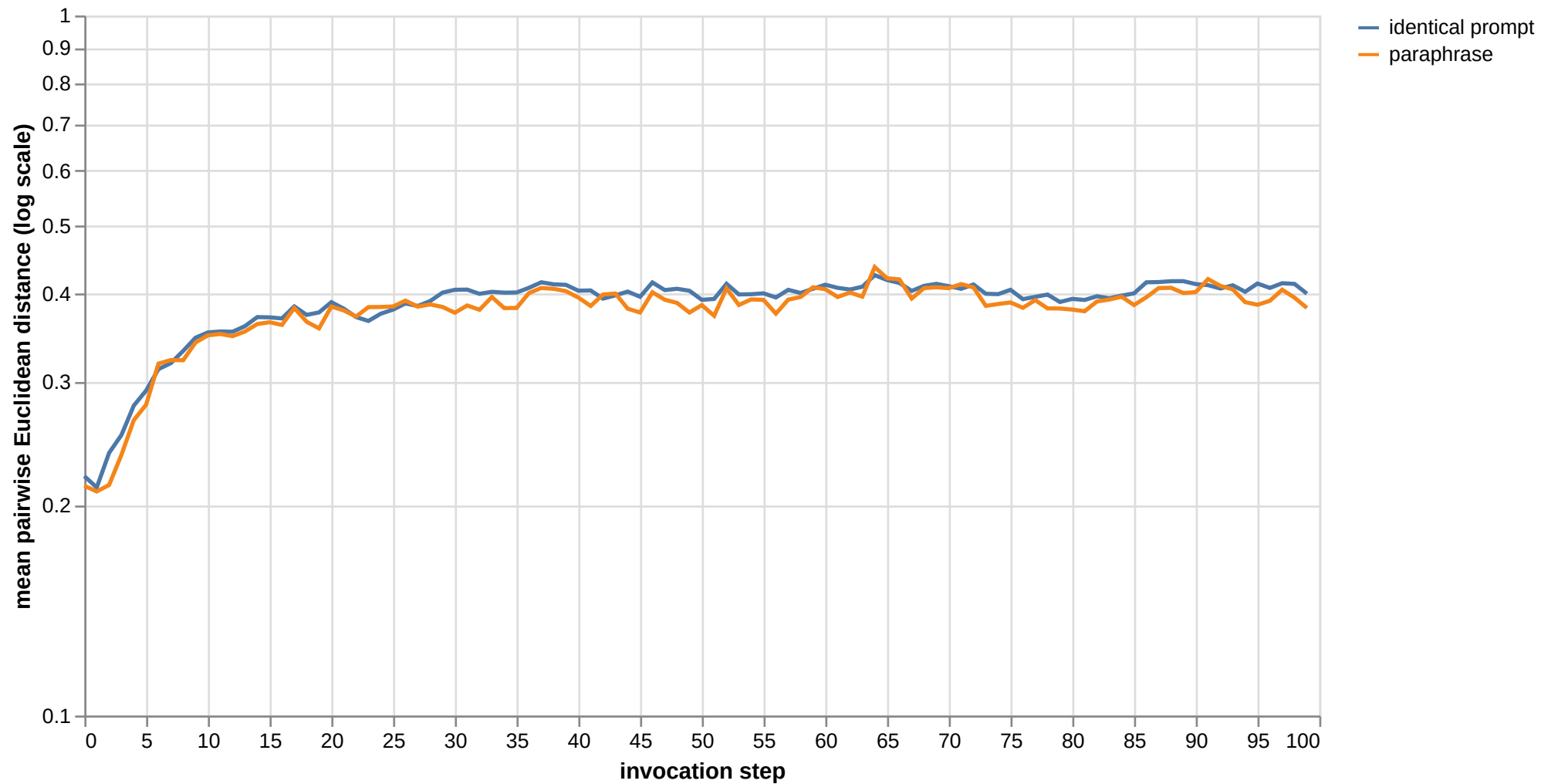
Divergence curve: SD35Medium → Pixtral · Qwen3Embed
