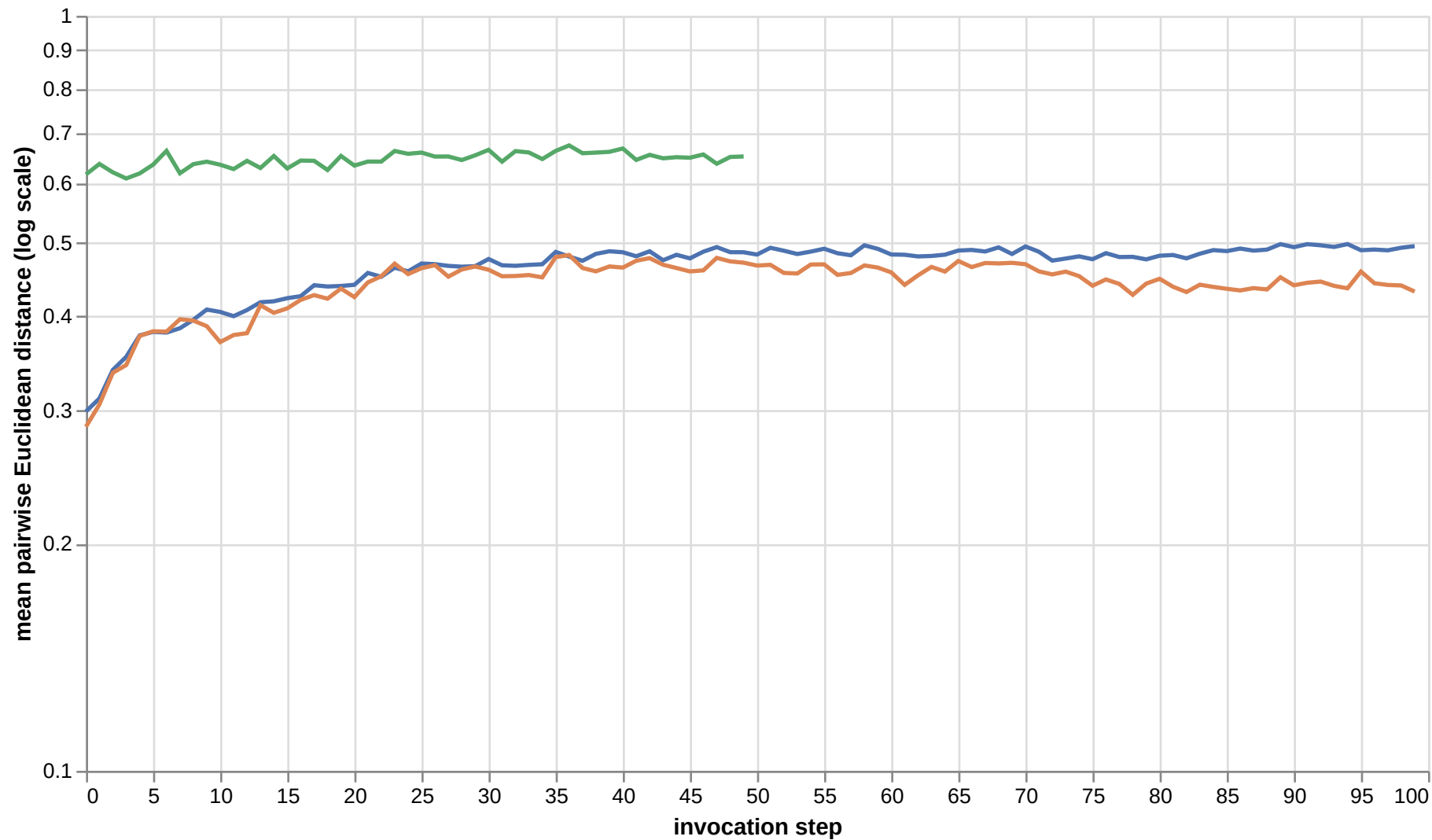
Three-regime divergence: Flux2Klein → Moondream · Qwen3Embed
