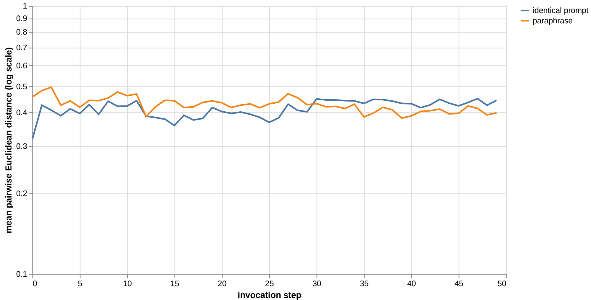
Divergence curve: QwenImage \rightarrow Pixtral \cdot Qwen3Embed
