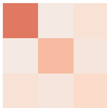
GLMImage → Gemma3n
