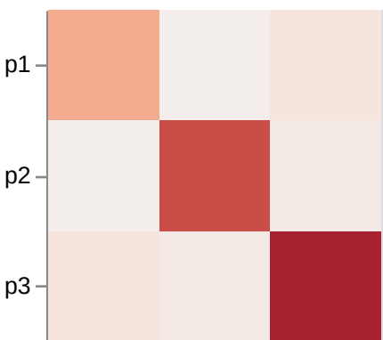
Flux2Klein → Moondream
