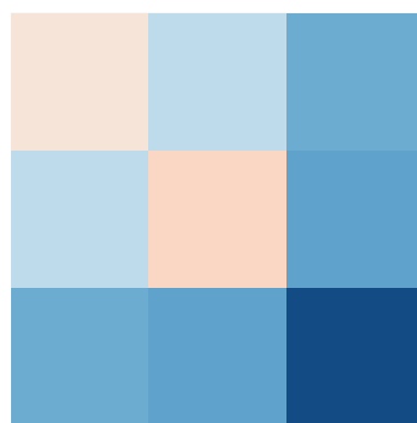
QwenImage → Qwen25VL
