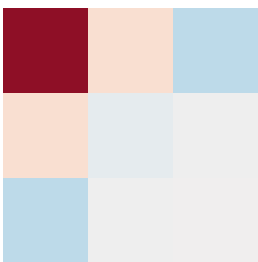
QwenImage → Pixtral
