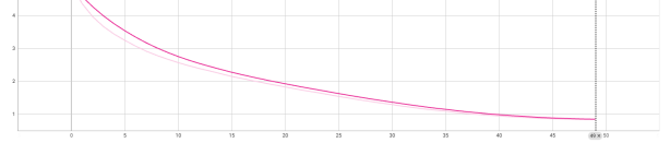
(f) Loss curve of ResNet18 on TinyImageNet
