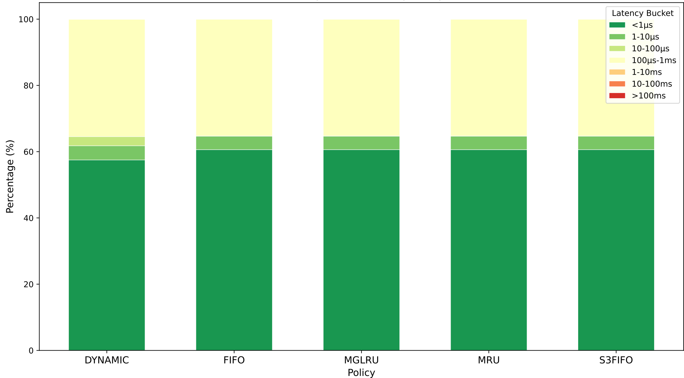
Latency Distribution by Policy
