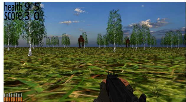
Figure 5: UI
