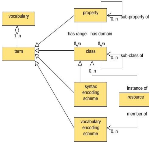
الشكل (4) : Class diagram for DCMI vocabulary model [21]
